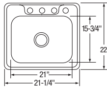
BOWL DEPTH: 6"
