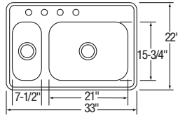
BOWL DEPTH: 8" (large) 5⅞" (small)
