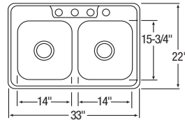
BOWL DEPTH: 8⅛"
